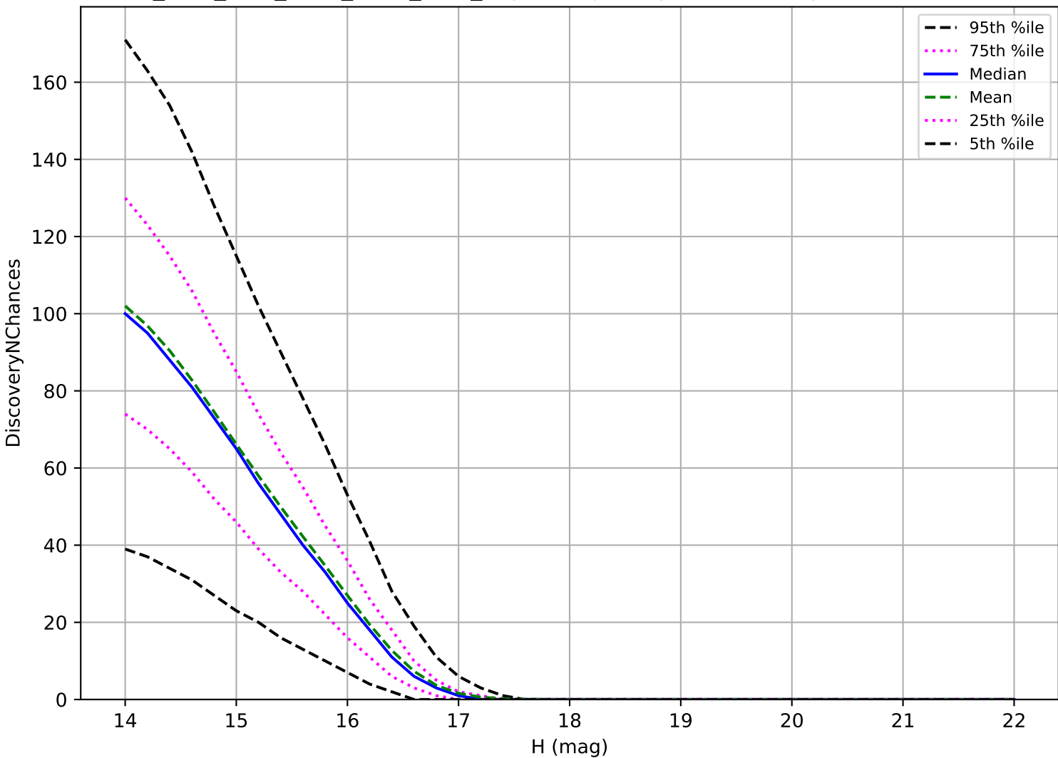
ddf_acor_sf20_lsf40_lsr20_v3.4_10yrs: Trojan 3 pairs in 15 nights detection loss
