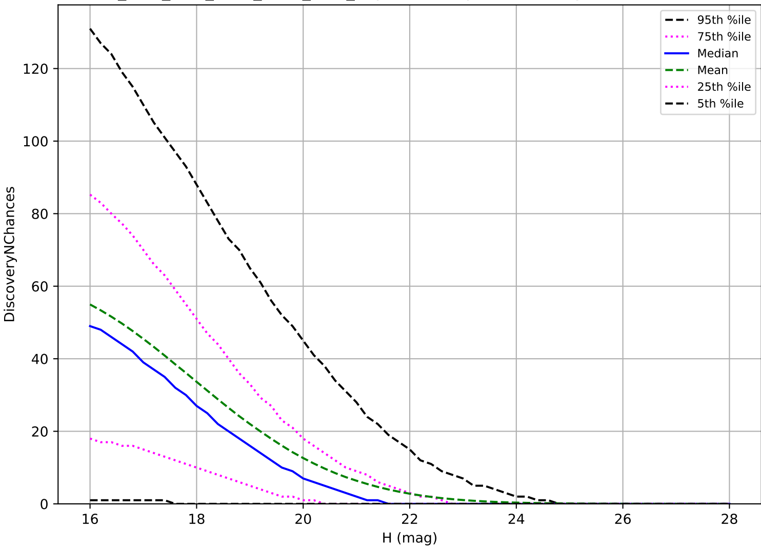
ddf_acor_sf20_lsf40_lsr20_v3.4_10yrs: PHA 3 pairs in 15 nights detection loss
