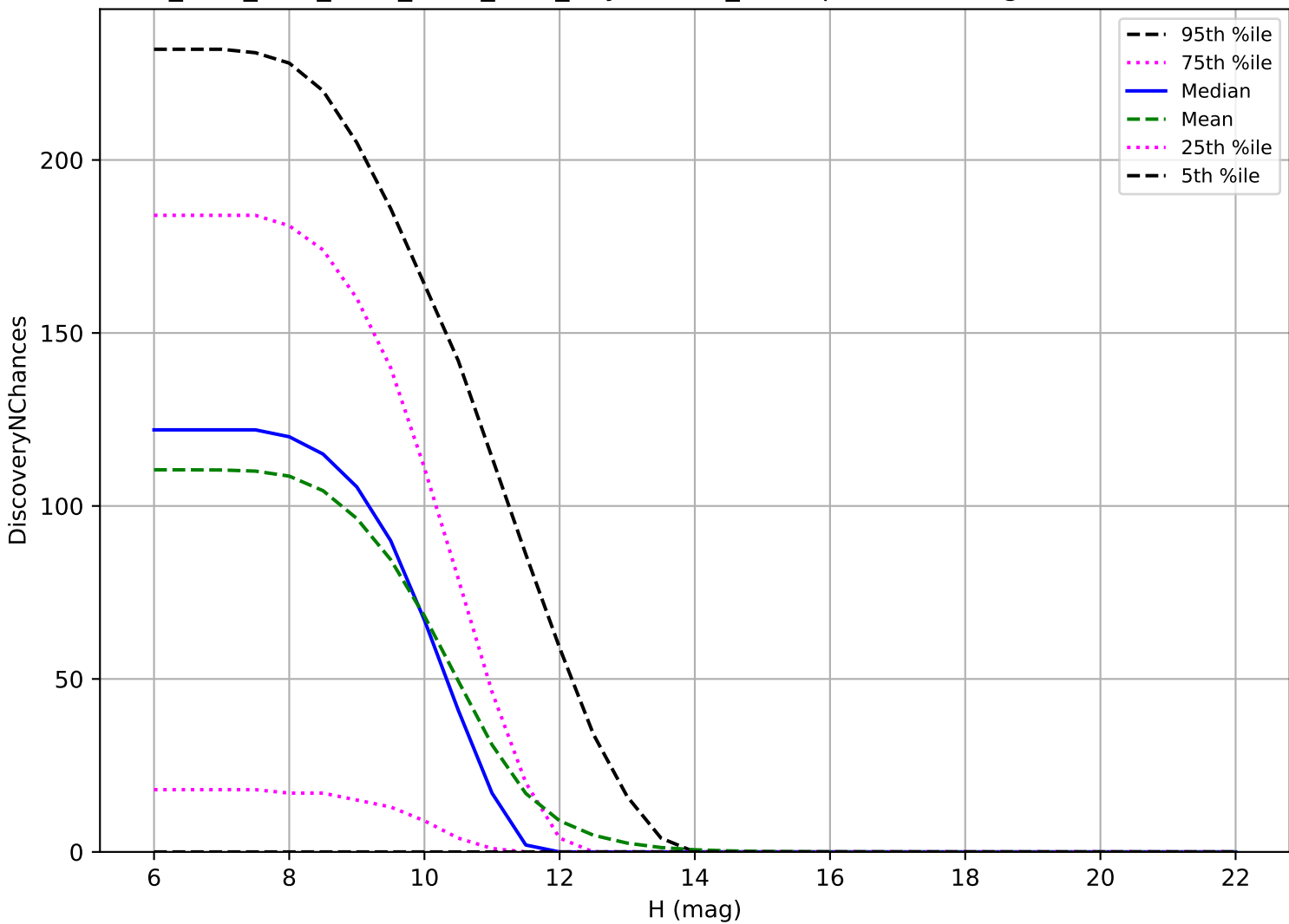
ddf_acor_sf20_lsf40_lsr20_v3.4_10yrs: OCC_r20 3 pairs in 15 nights detection loss
