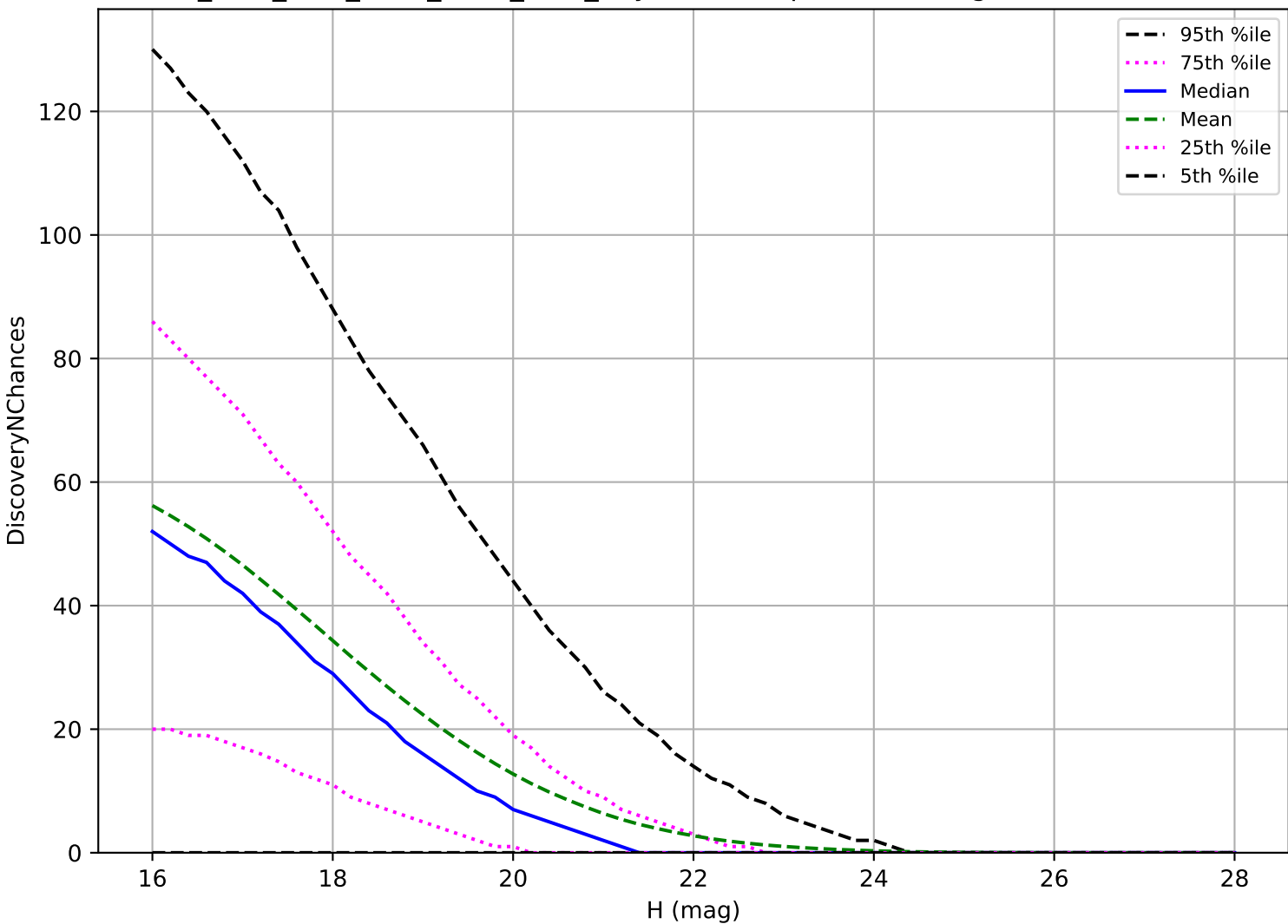
ddf_acor_sf20_lsf40_lsr20_v3.4_10yrs: NEO 3 pairs in 15 nights detection loss
