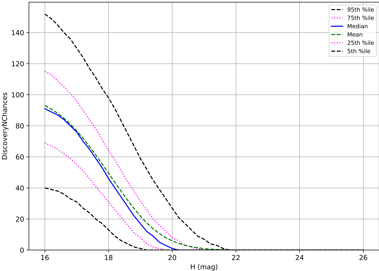
ddf_acor_sf20_lsf40_lsr20_v3.4_10yrs: MBA 3 pairs in 15 nights detection loss
