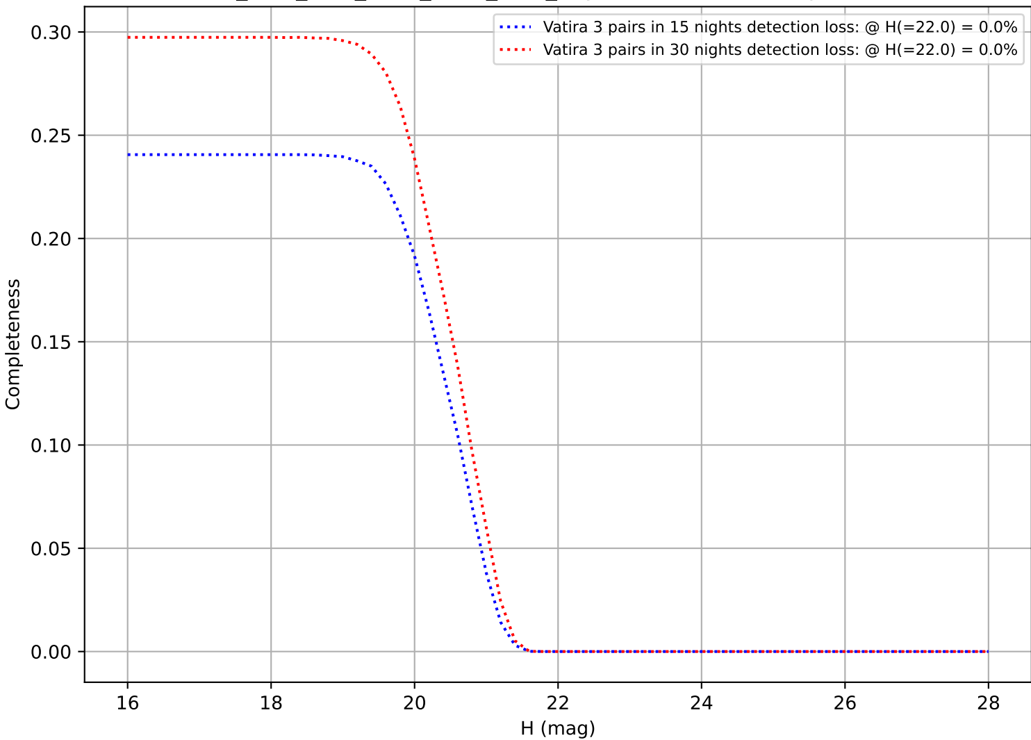
ddf_acor_sf20_lsf40_lsr20_v3.4_10yrs: DifferentialCompleteness
