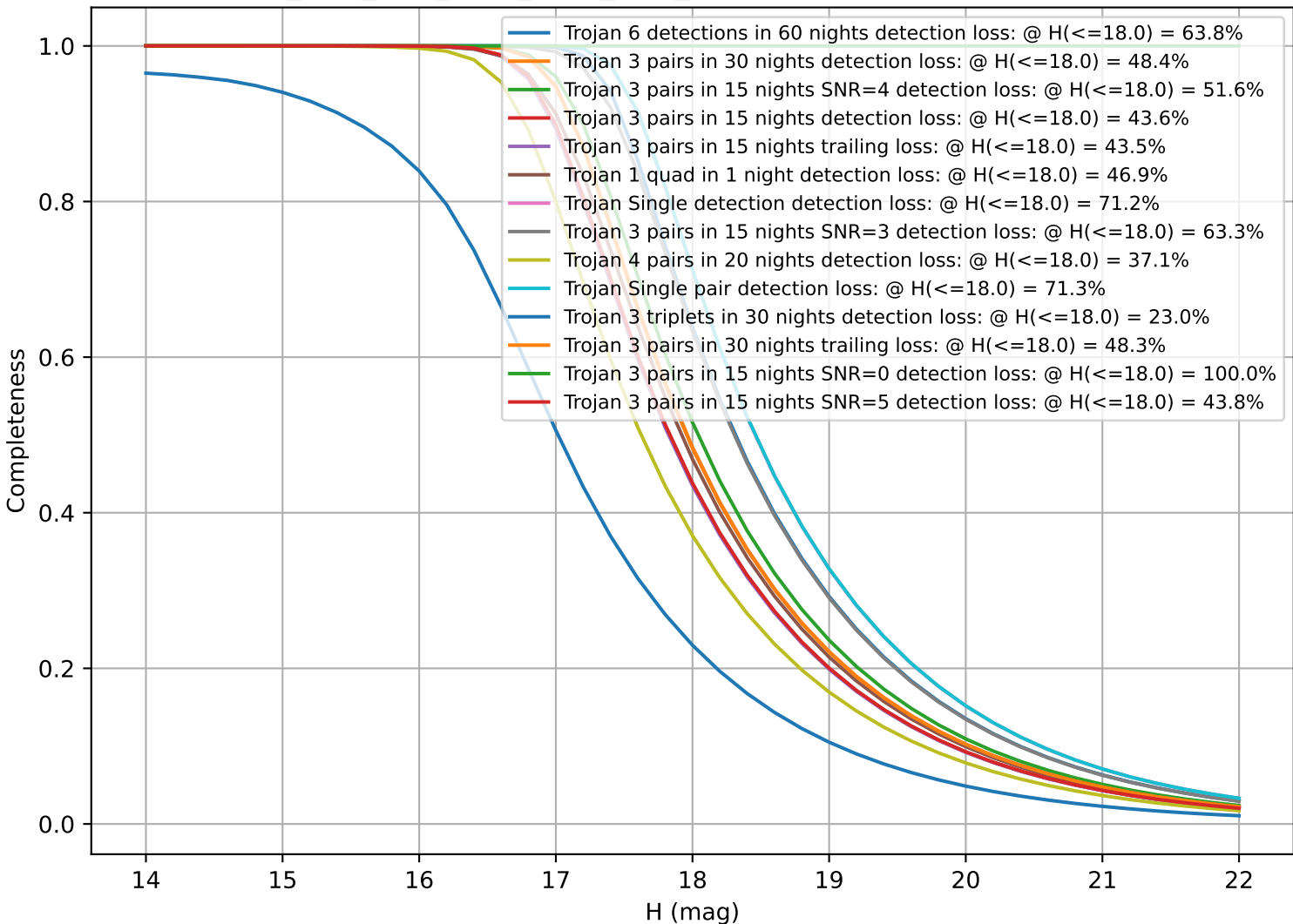
ddf_acor_sf20_lsf40_lsr20_v3.4_10yrs: CumulativeCompleteness
