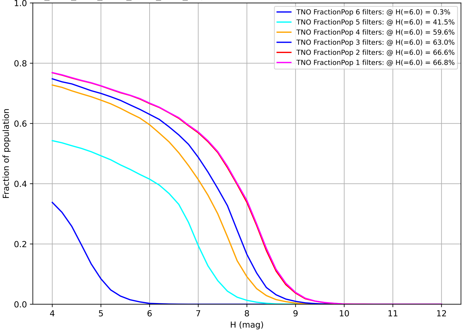
ddf_acor_sf20_lsf40_lsr20_v3.4_10yrs: Fraction of population with colors in X filters TNO
