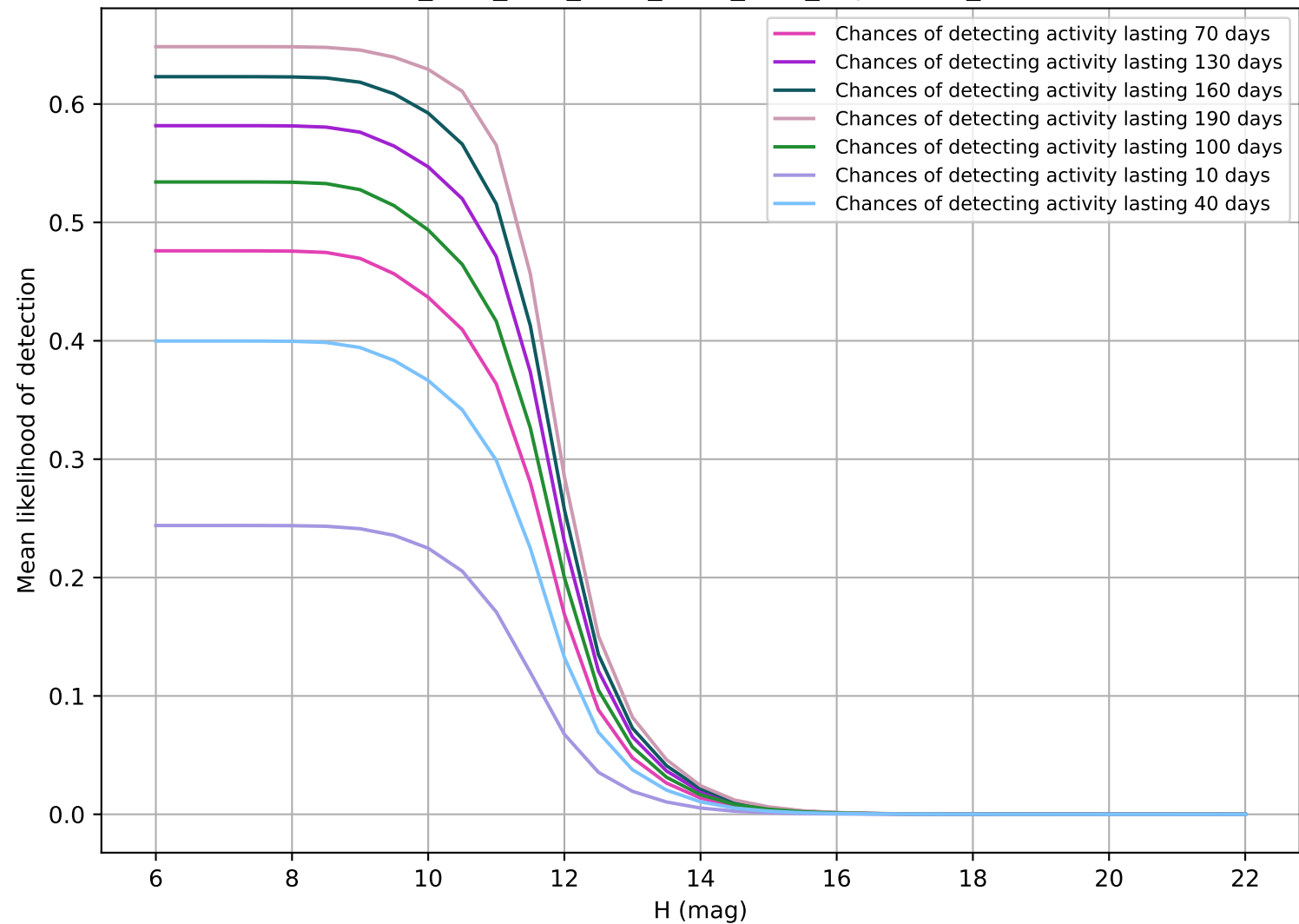
ddf_acor_sf20_lsf40_lsr20_v3.4_10yrs OCC_r20
