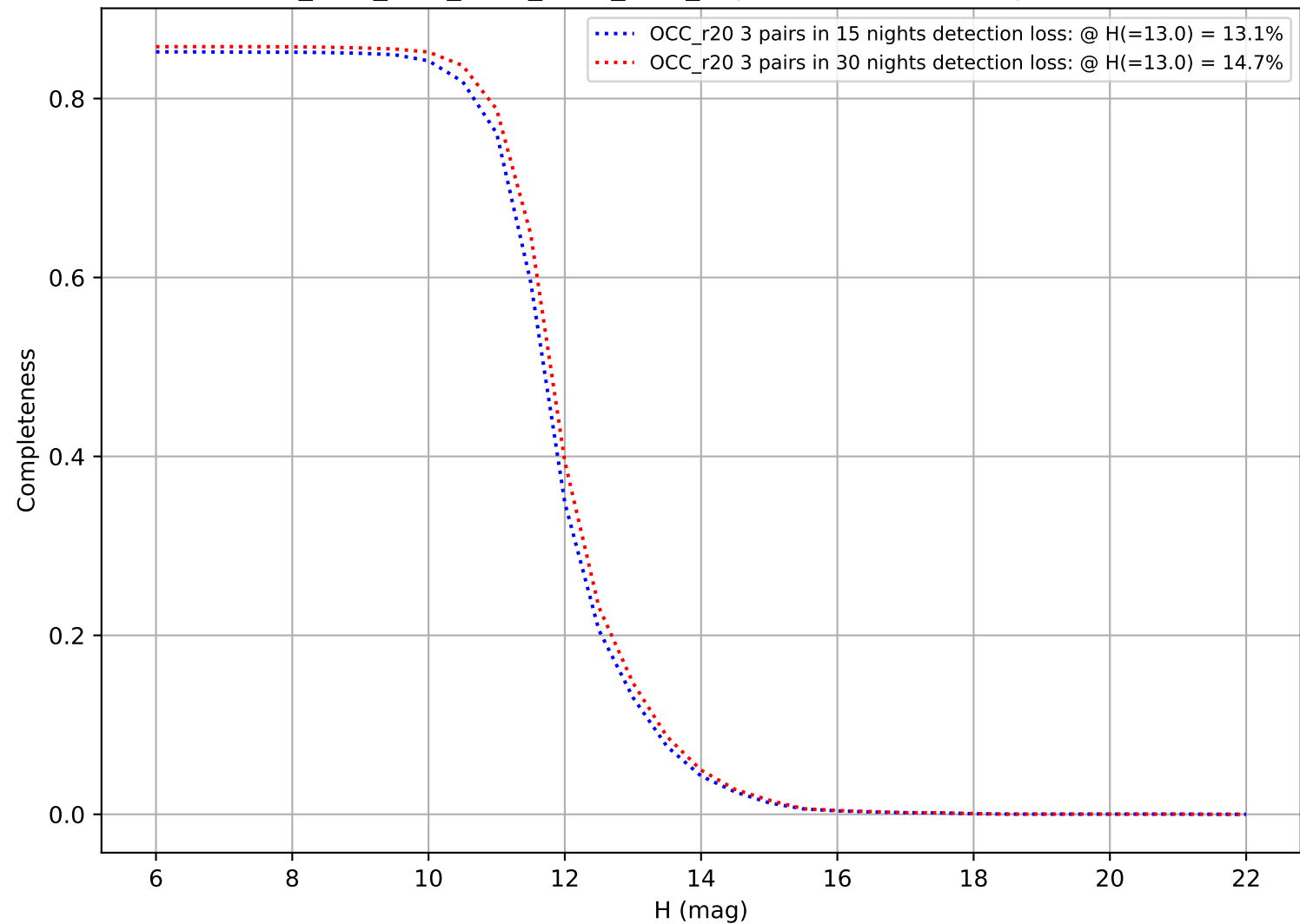
ddf_acor_sf20_lsf40_lsr20_v3.4_10yrs: DifferentialCompleteness
