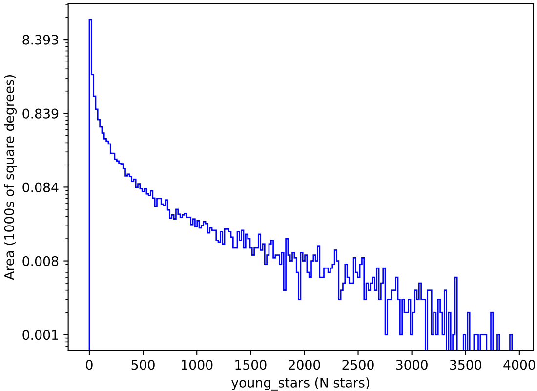
ddf_acor_sf20_lsf40_lsr20_v3.4_10yrs : young_stars
