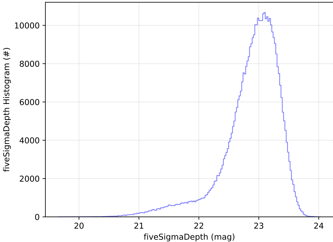
ddf_acor_sf20_lsf40_lsr20_v3.4_10yrs z: fiveSigmaDepth Histogram
