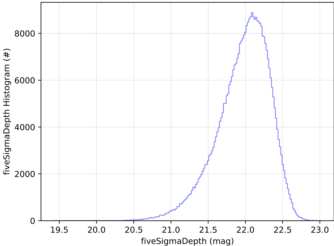
ddf_acor_sf20_lsf40_lsr20_v3.4_10yrs y: fiveSigmaDepth Histogram
