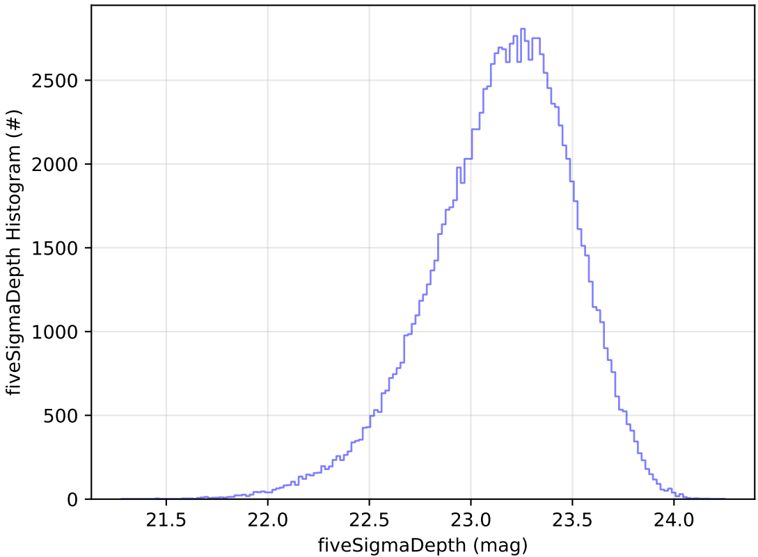
ddf_acor_sf20_lsf40_lsr20_v3.4_10yrs u: fiveSigmaDepth Histogram
