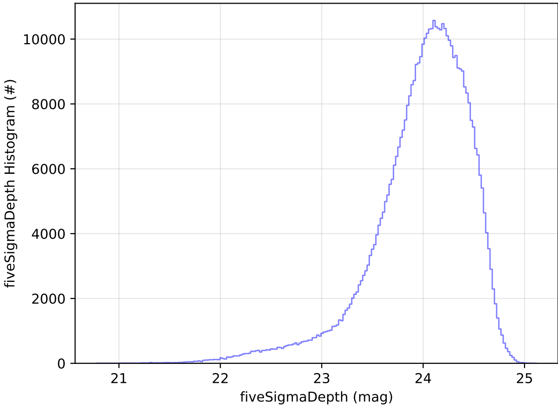
ddf_acor_sf20_lsf40_lsr20_v3.4_10yrs r: fiveSigmaDepth Histogram
