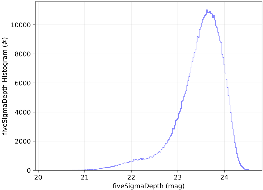
ddf_acor_sf20_lsf40_lsr20_v3.4_10yrs i: fiveSigmaDepth Histogram
