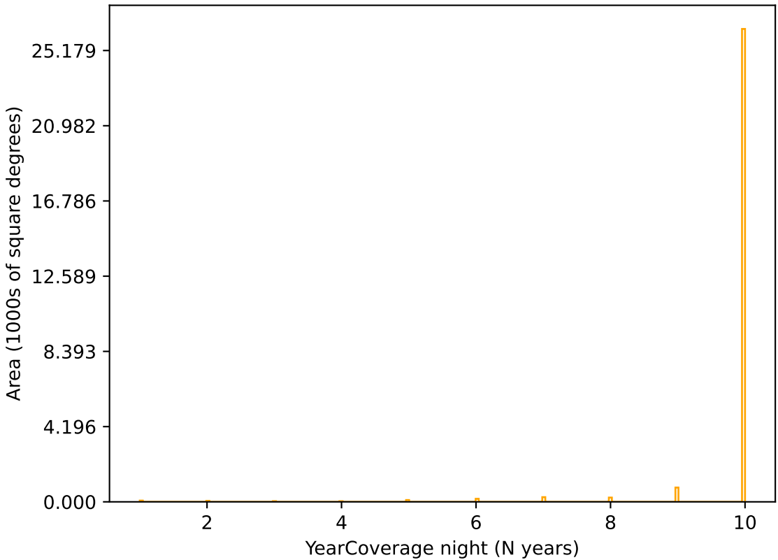
ddf_acor_sf20_lsf40_lsr20_v3.4_10yrs r band: YearCoverage night
