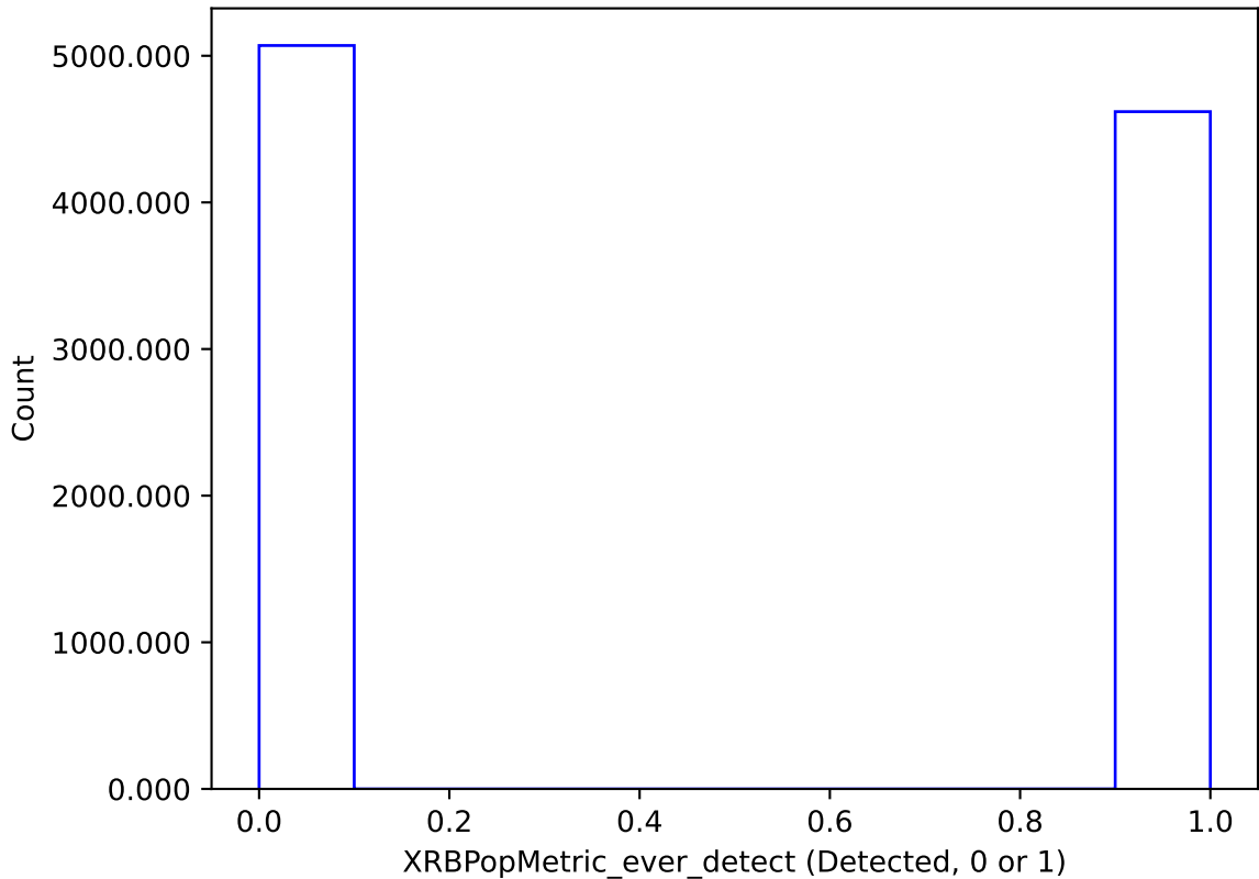
ddf_acor_sf20_lsf40_lsr20_v3.4_10yrs : XRBPoMetric_ever_detect
