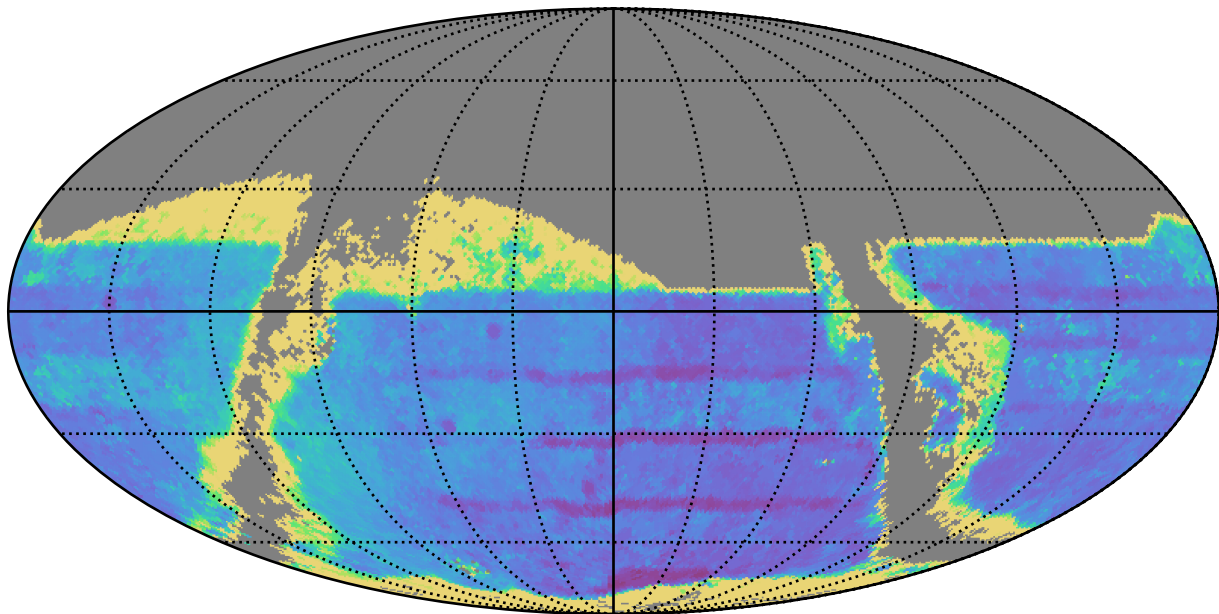
ddf_acor_sf20_lsf40_lsr20_v3.4_10yrs : TDC_accuracy
