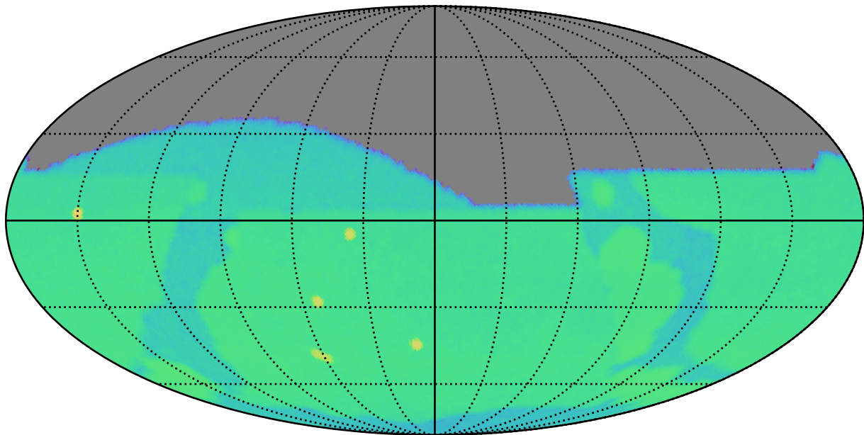
ddf_acor_sf20_lsf40_lsr20_v3.4_10yrs g: SurfaceBrightLimit
