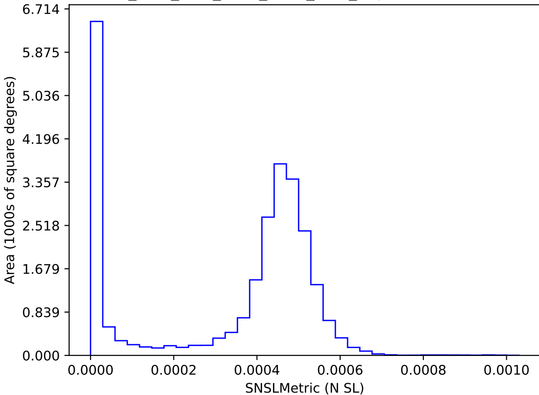
ddf_acor_sf20_lsf40_lsr20_v3.4_10yrs : SNSLMetric
