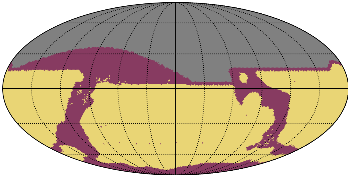
ddf_acor_sf20_lsf40_lsr20_v3.4_10yrs : RapidRevisits
