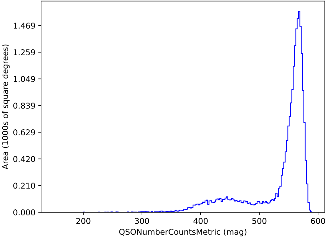
ddf_acor_sf20_lsf40_lsr20_v3.4_10yrs y band and non-DD: QSONumberCountsMetric
