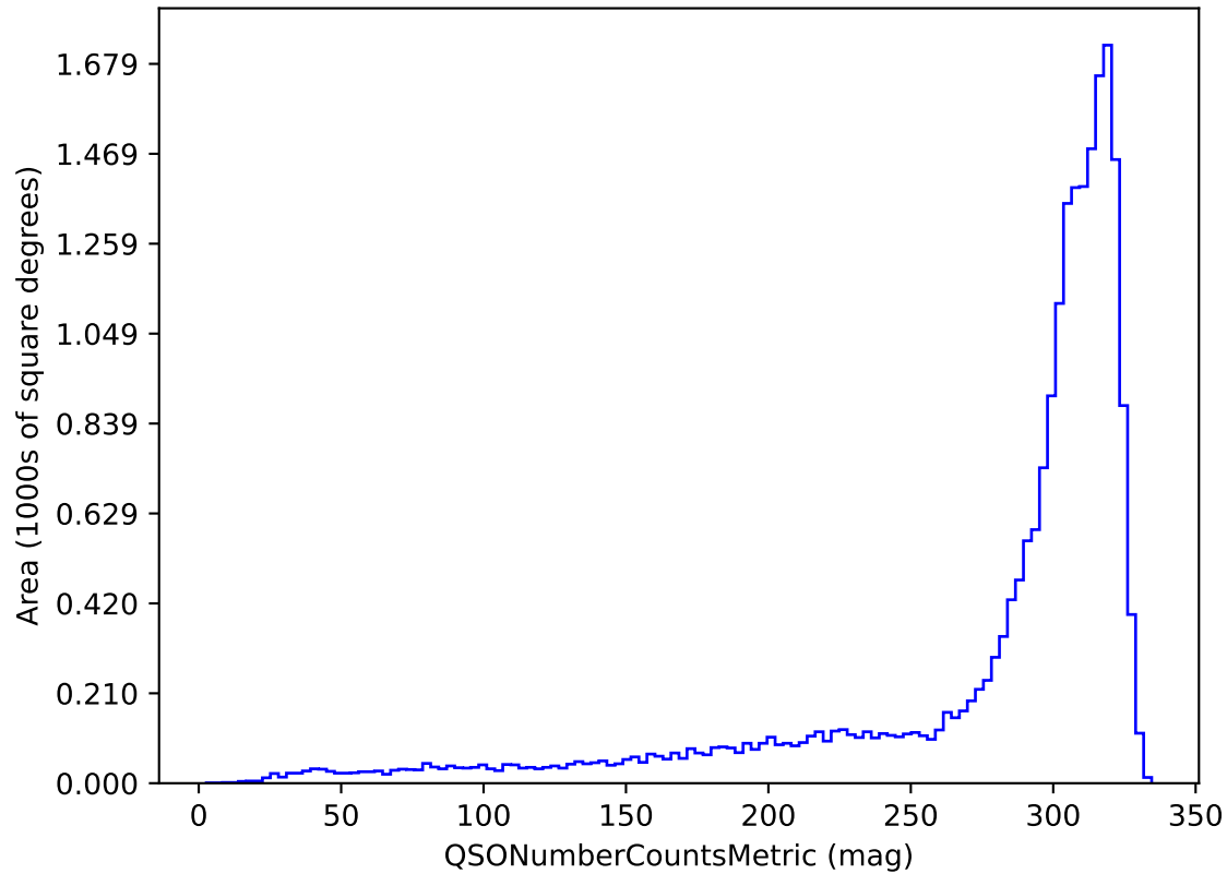
ddf_acor_sf20_lsf40_lsr20_v3.4_10yrs u band and non-DD: QSONumberCountsMetric
