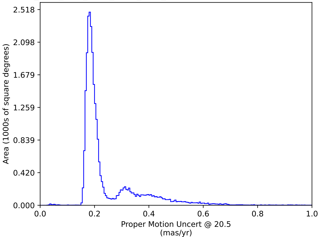
ddf_acor_sf20_lsf40_lsr20_v3.4_10yrs : Proper Motion Uncert @ 20.5
