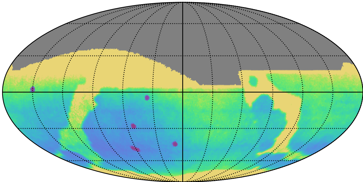
ddf_acor_sf20_lsf40_lsr20_v3.4_10yrs : Parallax Uncert @ 24.0
