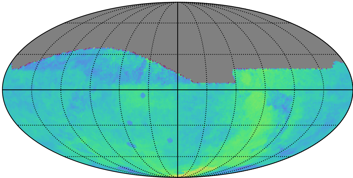
ddf_acor_sf20_lsf40_lsr20_v3.4_10yrs : Parallax Coverage @ 24.0
