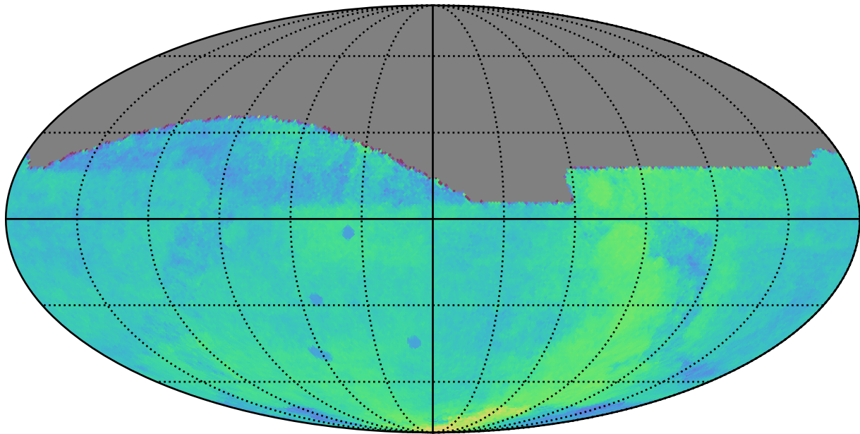
ddf_acor_sf20_lsf40_lsr20_v3.4_10yrs : Parallax Coverage @ 22.4
