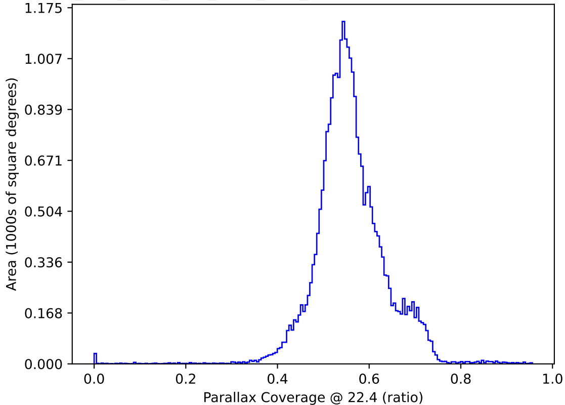
ddf_acor_sf20_lsf40_lsr20_v3.4_10yrs : Parallax Coverage @ 22.4
