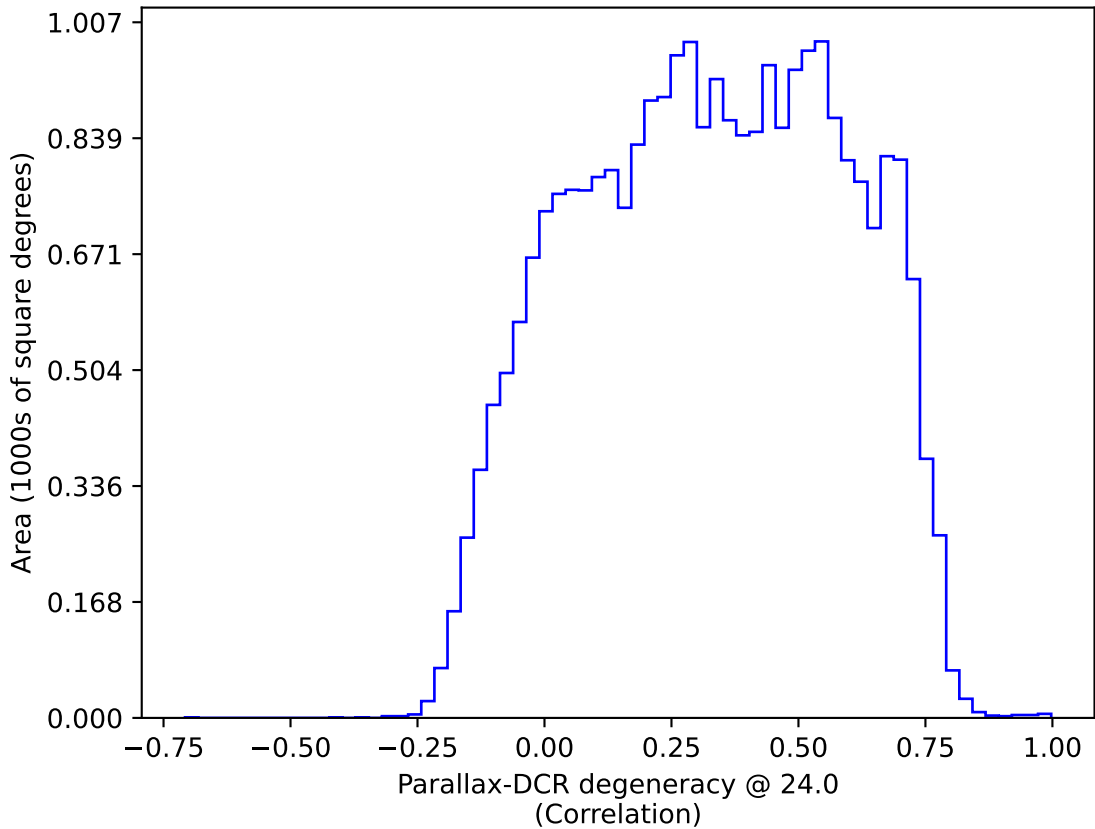
ddf_acor_sf20_lsf40_lsr20_v3.4_10yrs : Parallax-DCR degeneracy @ 24.0
