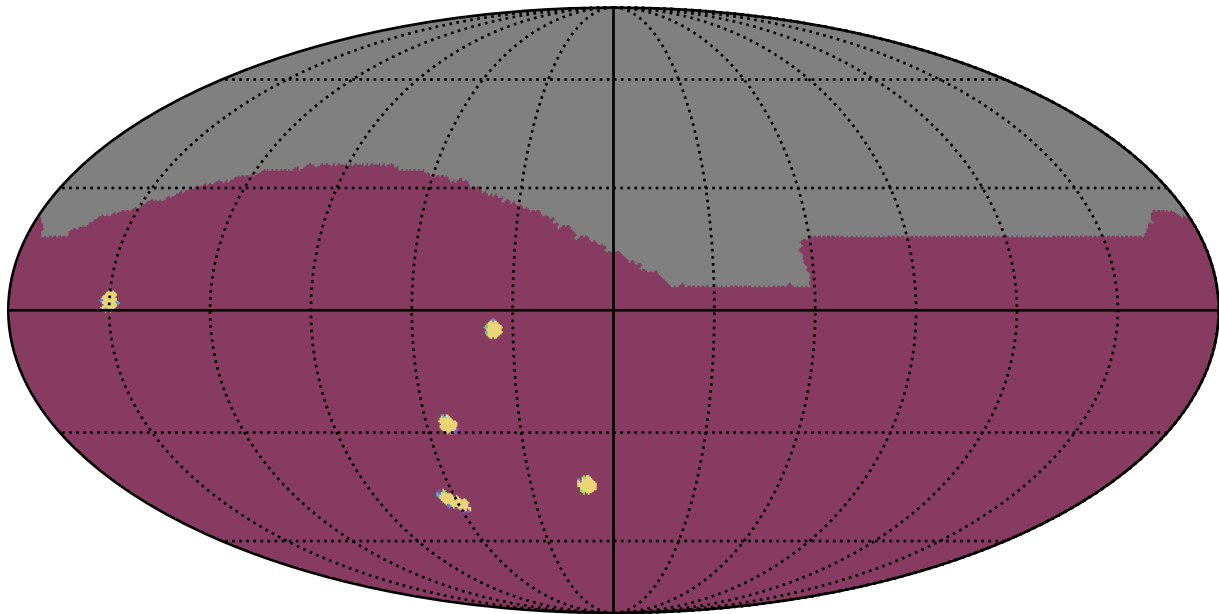
ddf_acor_sf20_lsf40_lsr20_v3.4_10yrs : NumberOfQuickRevisits
