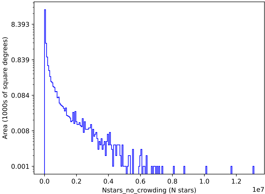
ddf_acor_sf20_lsf40_lsr20_v3.4_10yrs g: Nstars_no_crowding
