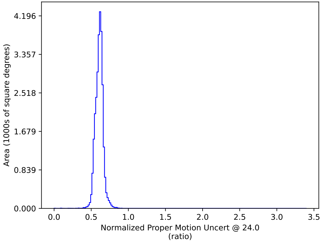
ddf_acor_sf20_lsf40_lsr20_v3.4_10yrs : Normalized Proper Motion Uncert @ 24.0
