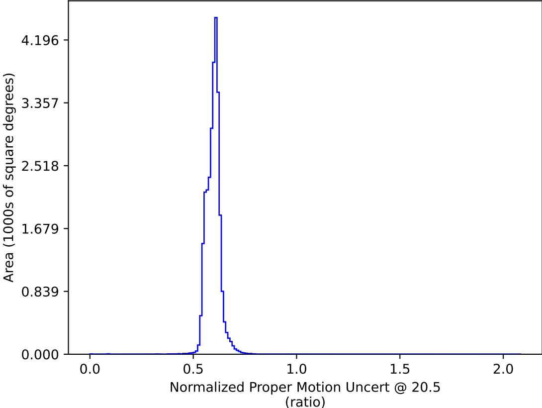
ddf_acor_sf20_lsf40_lsr20_v3.4_10yrs : Normalized Proper Motion Uncert @ 20.5
