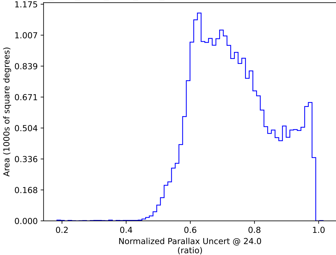
ddf_acor_sf20_lsf40_lsr20_v3.4_10yrs : Normalized Parallax Uncert @ 24.0
