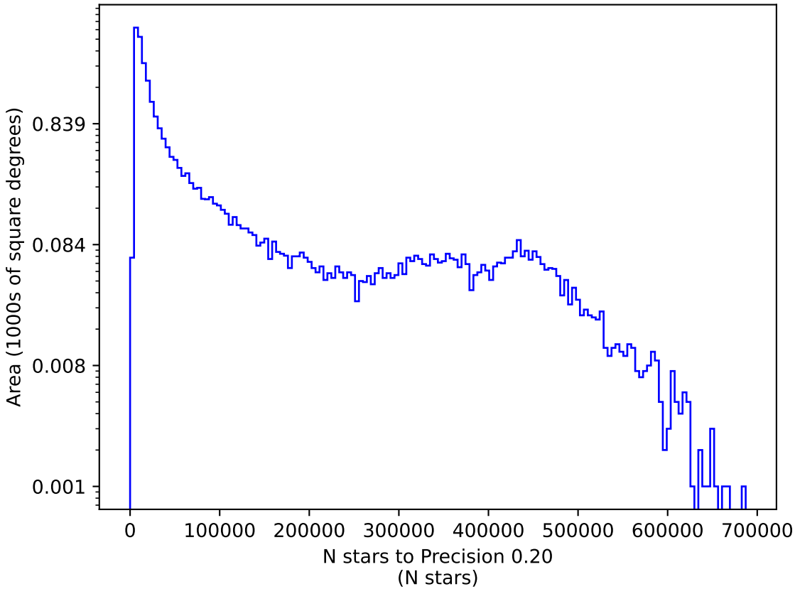
ddf_acor_sf20_lsf40_lsr20_v3.4_10yrs r: N stars to Precision 0.20
