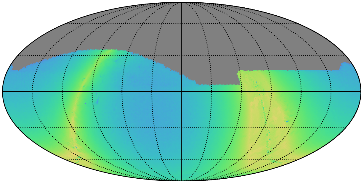
ddf_acor_sf20_lsf40_lsr20_v3.4_10yrs i: N stars to Precision 0.20
