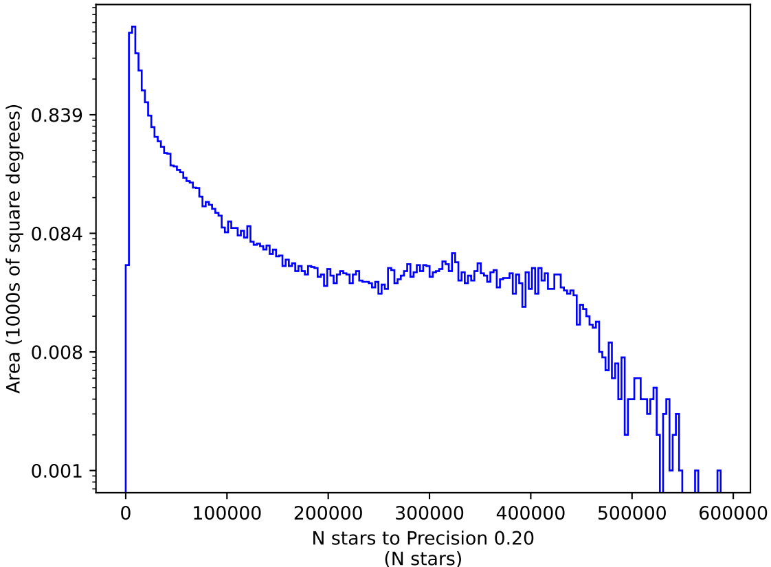
ddf_acor_sf20_lsf40_lsr20_v3.4_10yrs g: N stars to Precision 0.20
