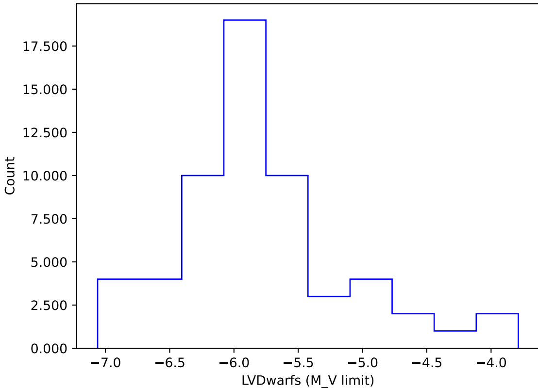
ddf_acor_sf20_lsf40_lsr20_v3.4_10yrs gi: LVDwarfs
