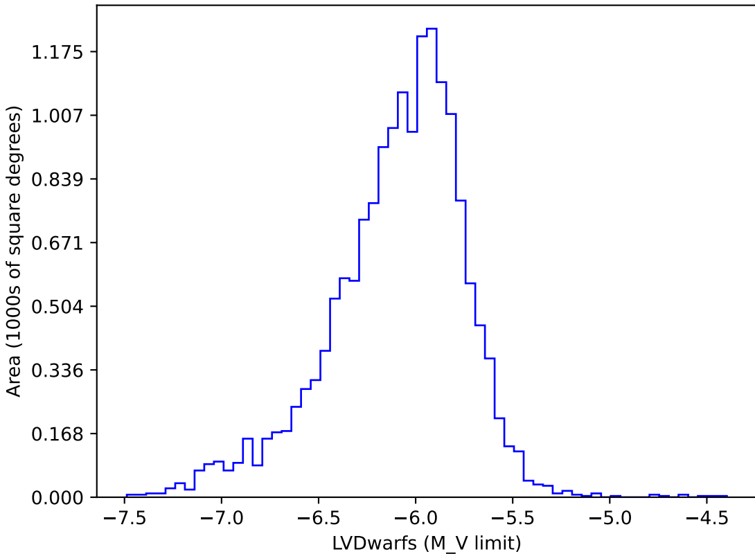
ddf_acor_sf20_lsf40_lsr20_v3.4_10yrs gi: LVDwarfs
