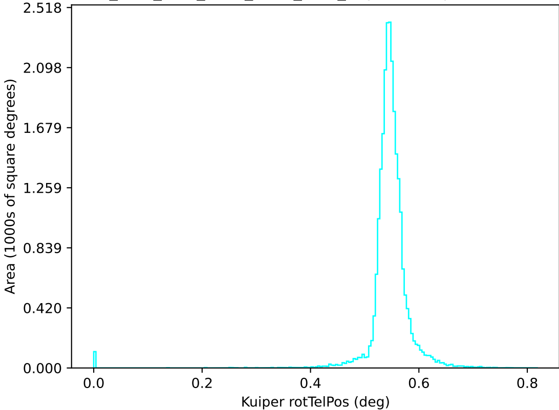
ddf_acor_sf20_ls40_lsr20_v3.4_10yrs u: Kuiper rotTelPos
