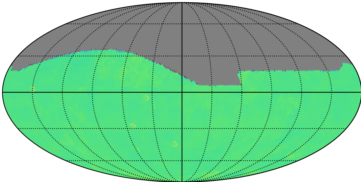
ddf_acor_sf20_lsf40_lsr20_v3.4_10yrs r: Kuiper rotTelPos
