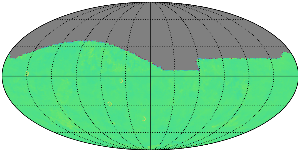
ddf_acor_sf20_lsf40_lsr20_v3.4_10yrs i: Kuiper rotTelPos
