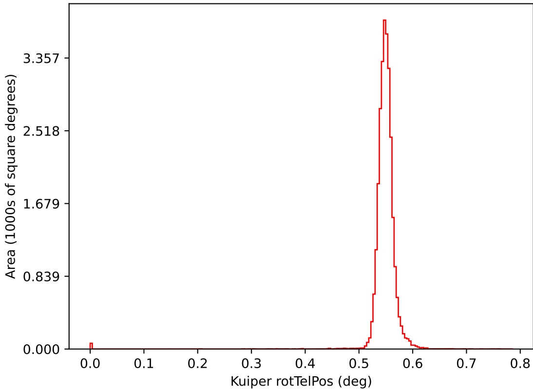
ddf_acor_sf20_lsf40_lsr20_v3.4_10yrs i: Kuiper rotTelPos
