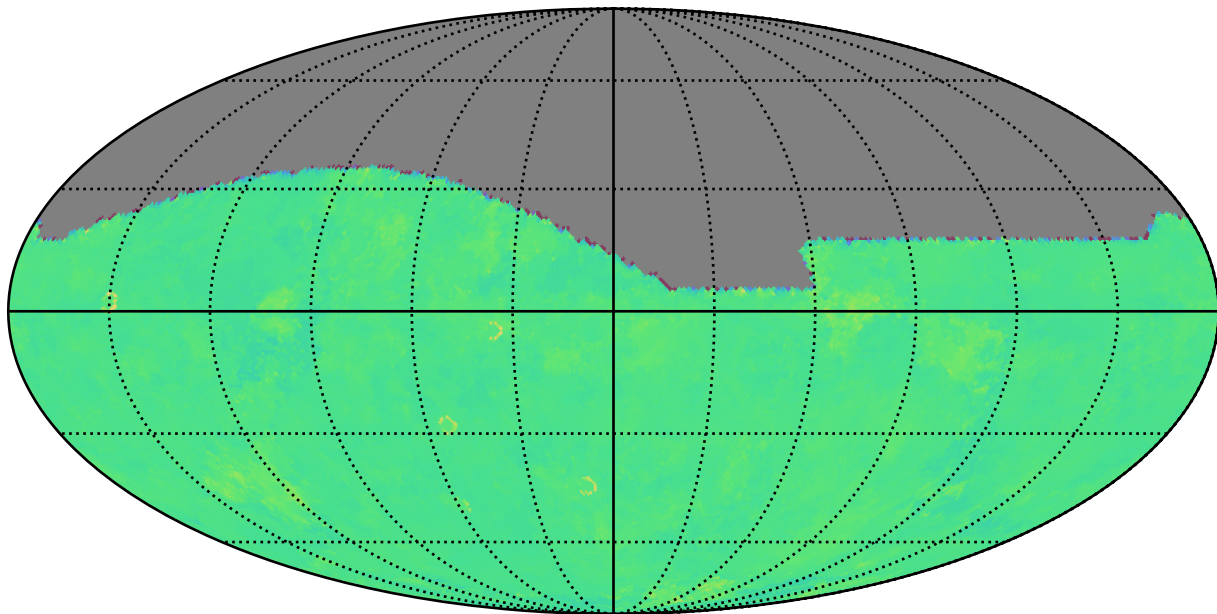
ddf_acor_sf20_lsf40_lsr20_v3.4_10yrs g: Kuiper rotTelPos
