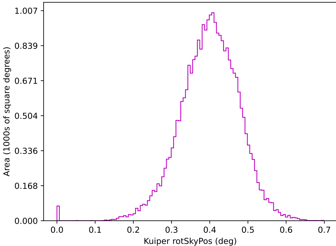
ddf_acor_sf20_lsf40_lsr20_v3.4_10yrs z: Kuiper rotSkyPos
