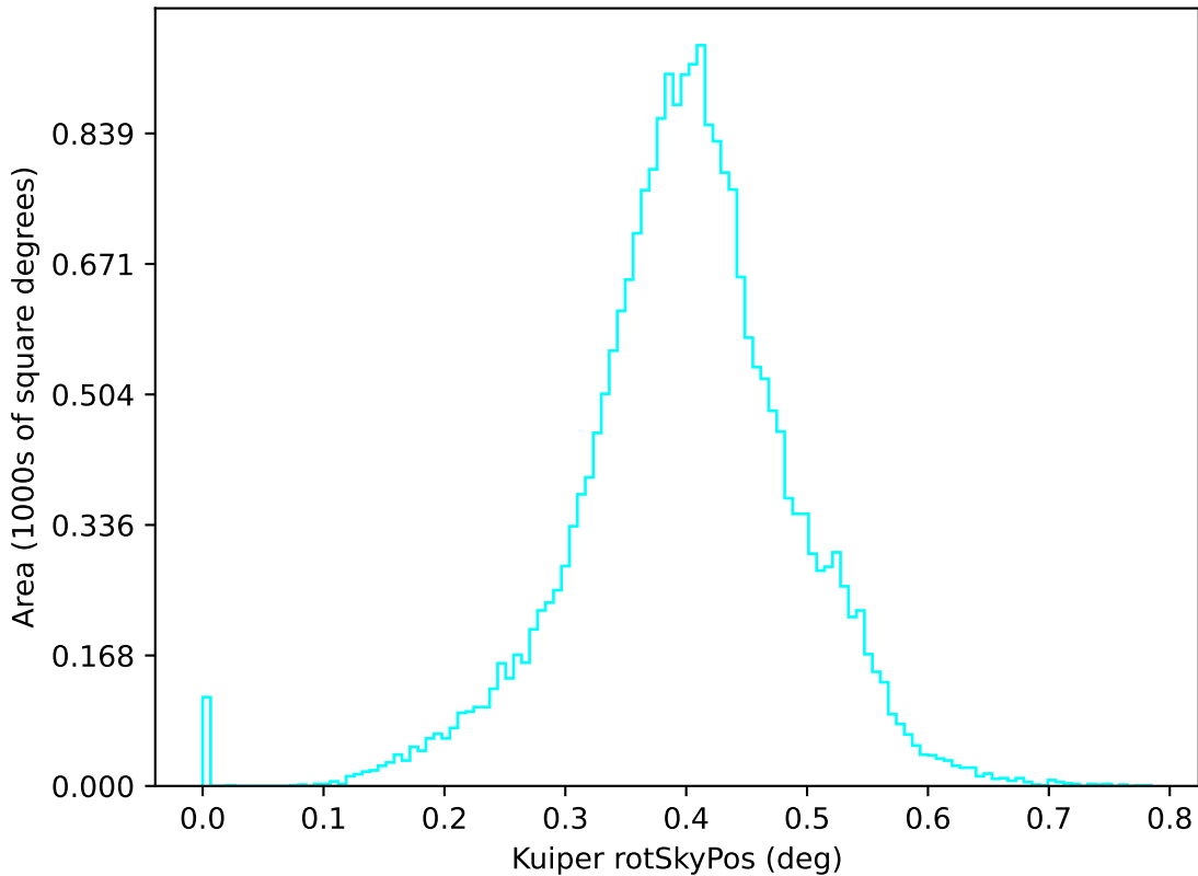
ddf_acor_sf20_lsf40_lsr20_v3.4_10yrs u: Kuiper rotSkyPos
