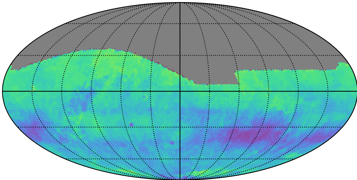
ddf_acor_sf20_lsf40_lsr20_v3.4_10yrs r: Kuiper rotSkyPos
