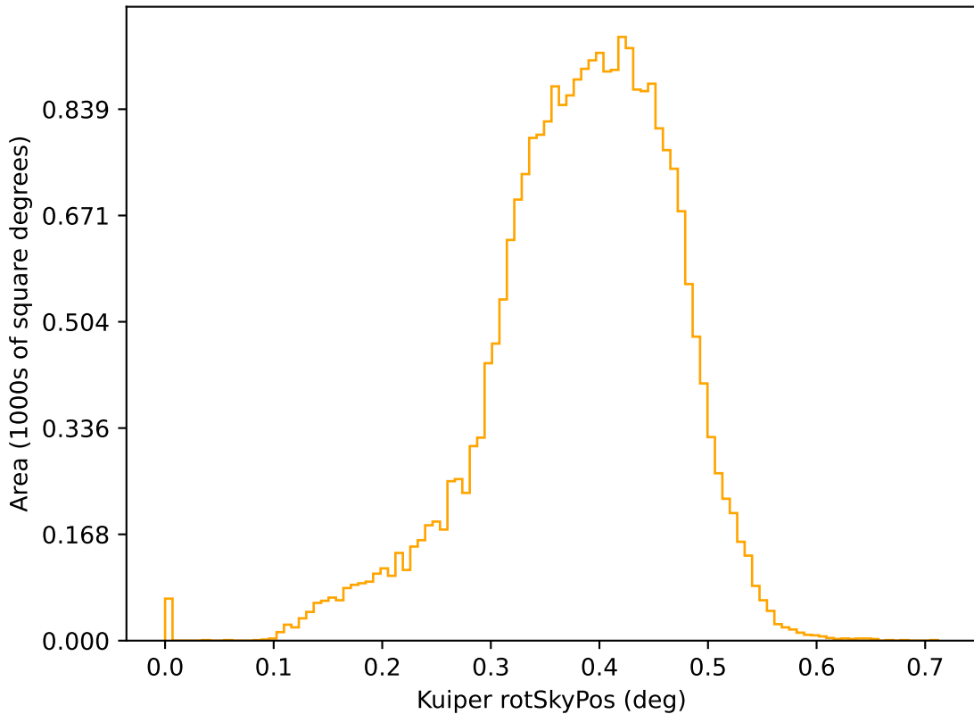
ddf_acor_sf20_lsf40_lsr20_v3.4_10yrs r: Kuiper rotSkyPos
