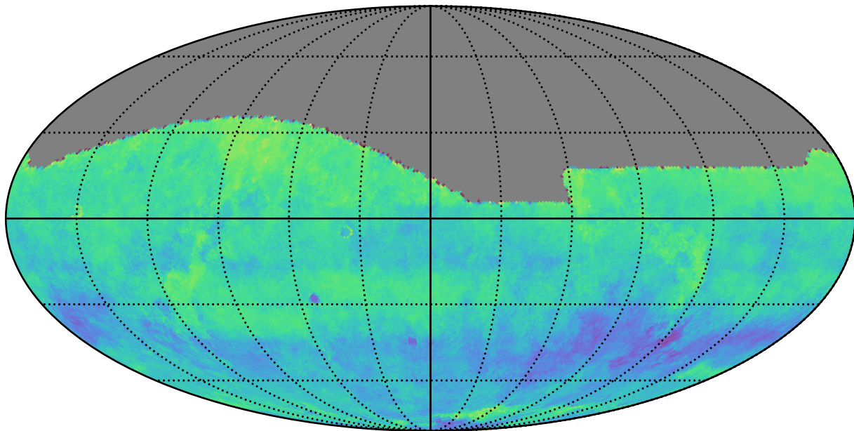
ddf_acor_sf20_lsf40_lsr20_v3.4_10yrs i: Kuiper rotSkyPos
